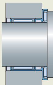
AXW series bearing combined with a drawn cup needle roller bearing
