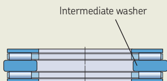
Double direction bearing, housing centred
