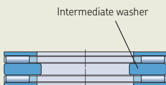
Double direction bearing, shaft centred
