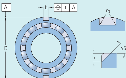
Locating slots in the outer ring of four-point contact ball bearings
