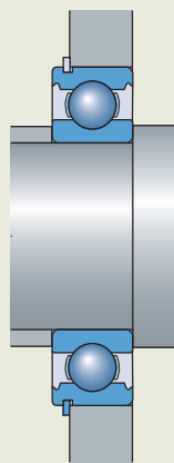
Bearing with a snap ring
